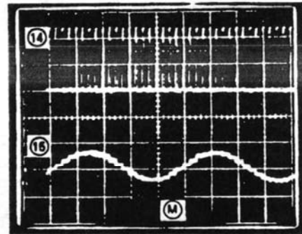
⑭ \mu PD833AC (M) SH signal PCB M5154-MA1M \mu PD833AC (M) pin 13 0.1 \mu S/div, 0.2V/div ⑮ Sample/Hold circuit output PCB M5154-MA1M TL082-2 pin 7 0.1 \mu S/div, 2V/div
