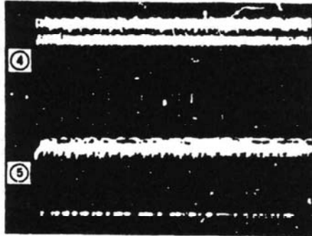
④ \mu PD7810H \overline{WR} signal PCB M5154-MA1M \mu PD7810H (SUB) pin 45 5 \mu S/div, 0.2V/div ⑤ \mu PD4454C \overline{CE} signal PCB M5154-MA1M \mu PD4454C-15L-1 pin 20 5 \mu S/div, 0.2V/div
