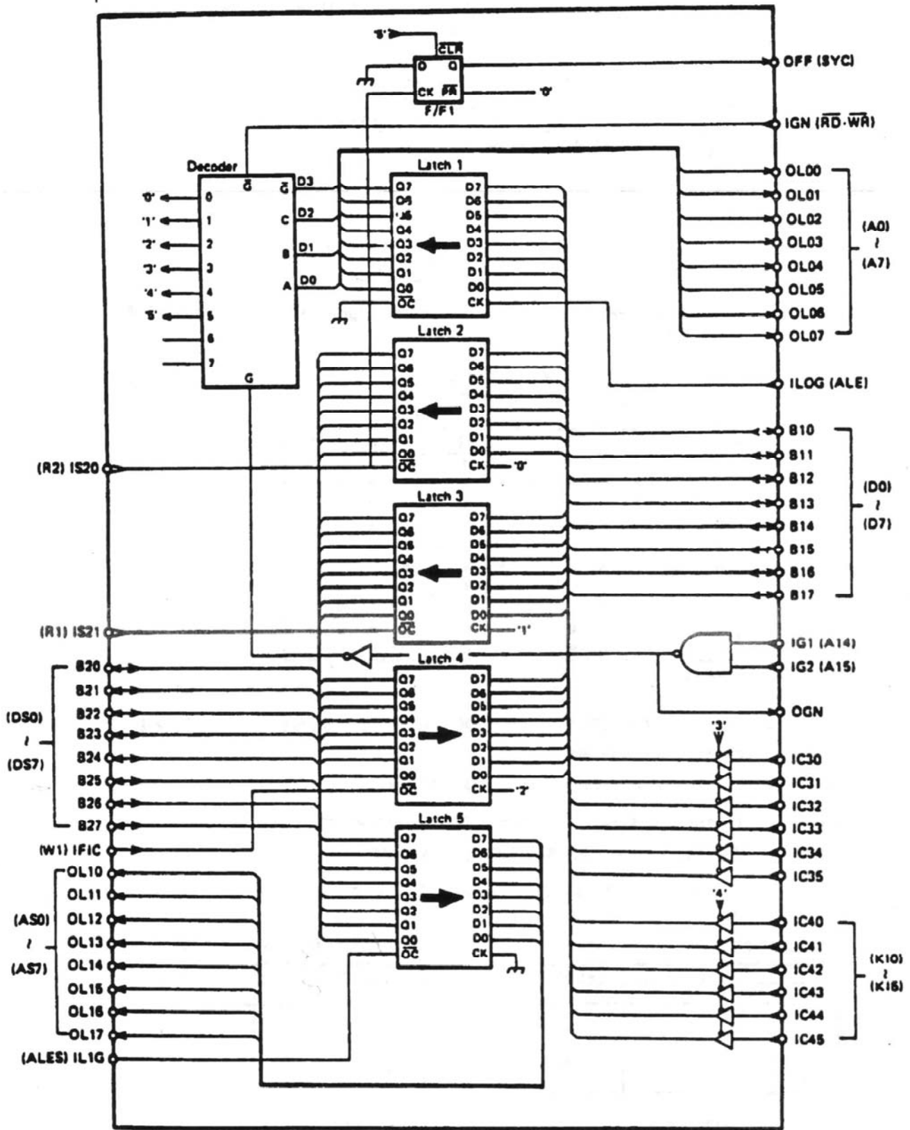
Internal block diagram of MB84H173
