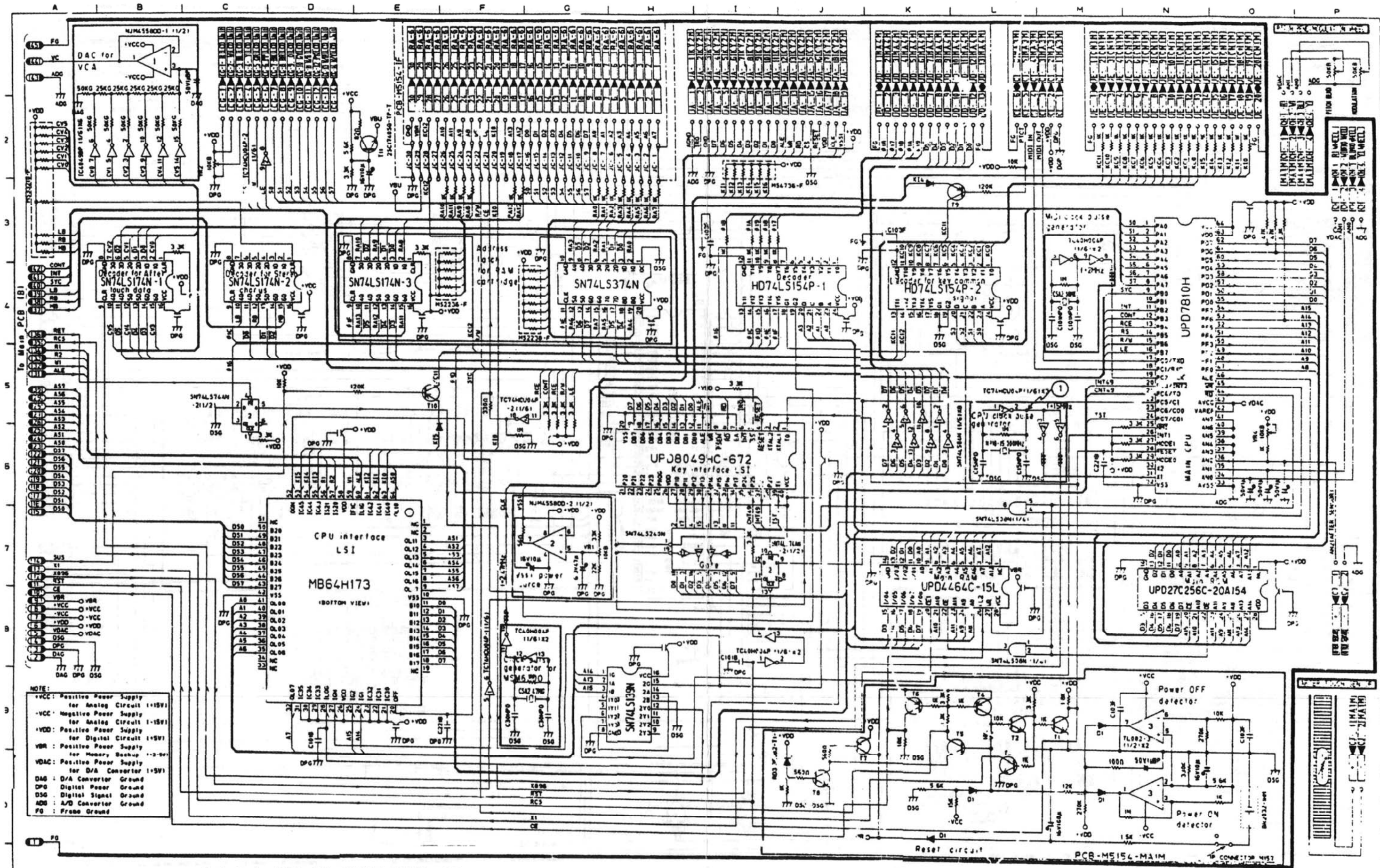
1-1 Main PCB (A) M5154-MA1M, IF
