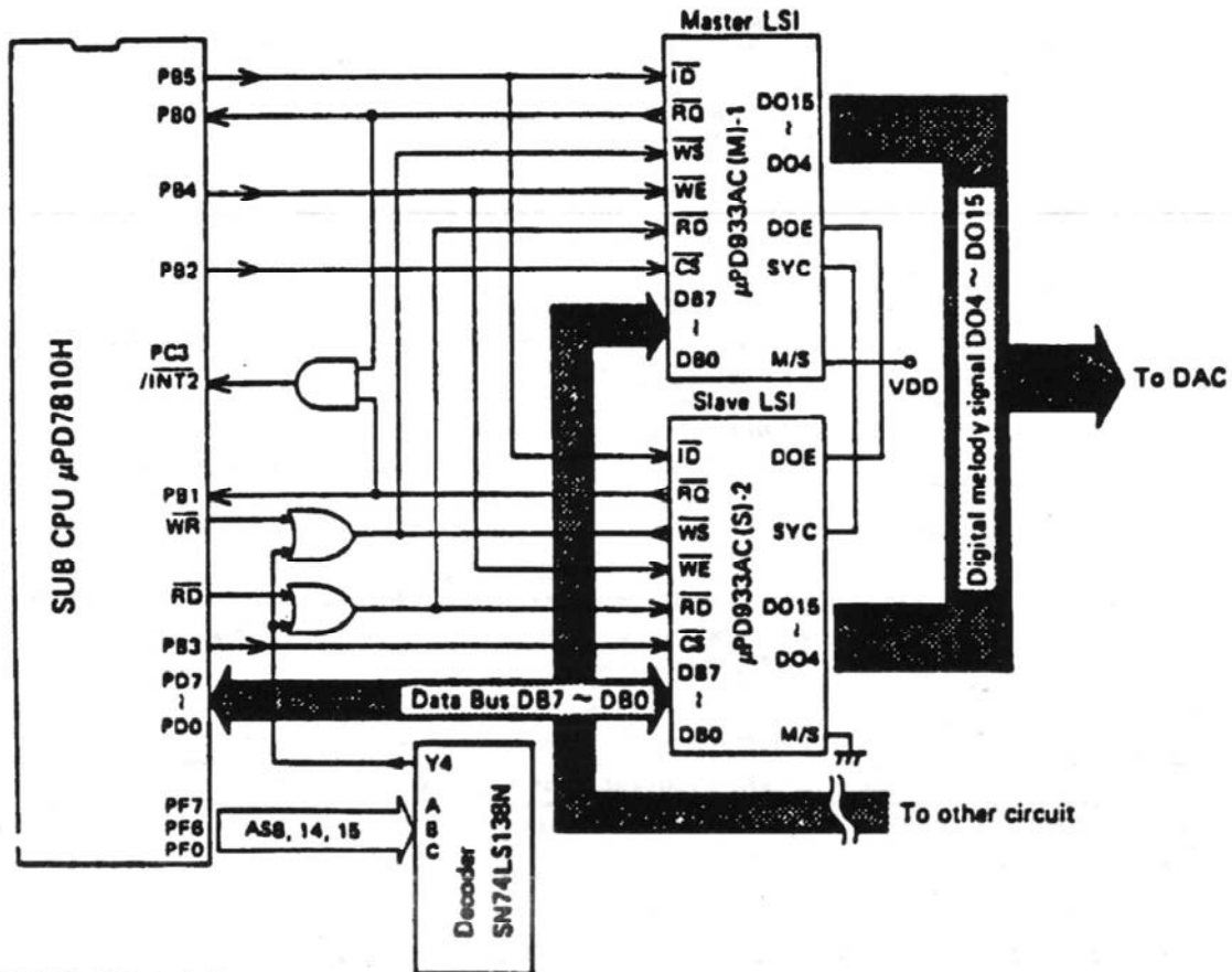
(1) SUB CPU \leftrightarrow Music LSI
