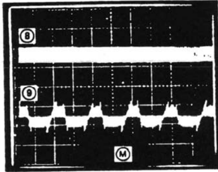
⑧ \mu PD833AC DOE signal PCB M5154-MA1M \mu PD833AC pin 12 2mS/div, 0.5V/div ⑨ DAC output PCB M5154-MA1M TL082-1 pin 1 10 \mu S/div, 0.5V/div
