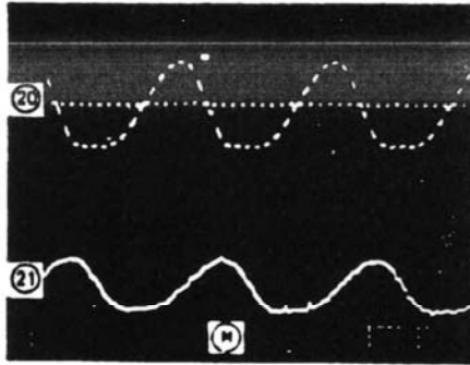
⑭ DAC output PCB M5154-MA1M TL082-1 pin 1 0.5mS/div, 0.2V/div
