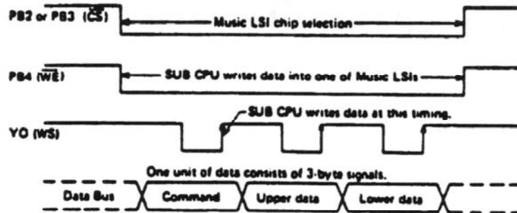
(2) Music LSI \rightarrow SUB CPU
