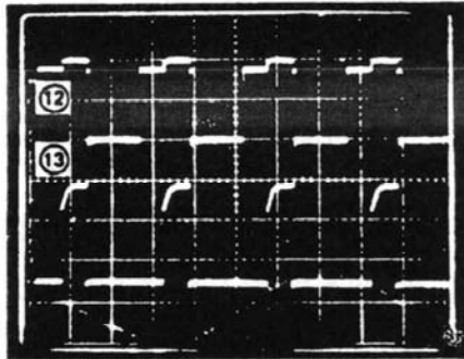
⑫ \mu PD833AC (M) DOE signal PCB M5154-MA1M \mu PD833AC (M) pin 12 10 \mu S/div, 0.2V/div ⑬ \mu PD833AC (M) SH signal PCB M5154-MA1M \mu PD833AC (M) pin 13 10 \mu S/div, 0.2V/div
