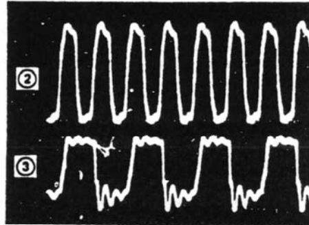
② \mu PD8049HC clock pulse PCB M5154-MA1M TC74HC04P-1 pin 11 0.1 \mu S/div, 0.2V/div ③ \mu PD833AC clock pulse PCB M5154-MA1M \mu PD833AC pin 8 0.1 \mu S/div, 0.2V/div
