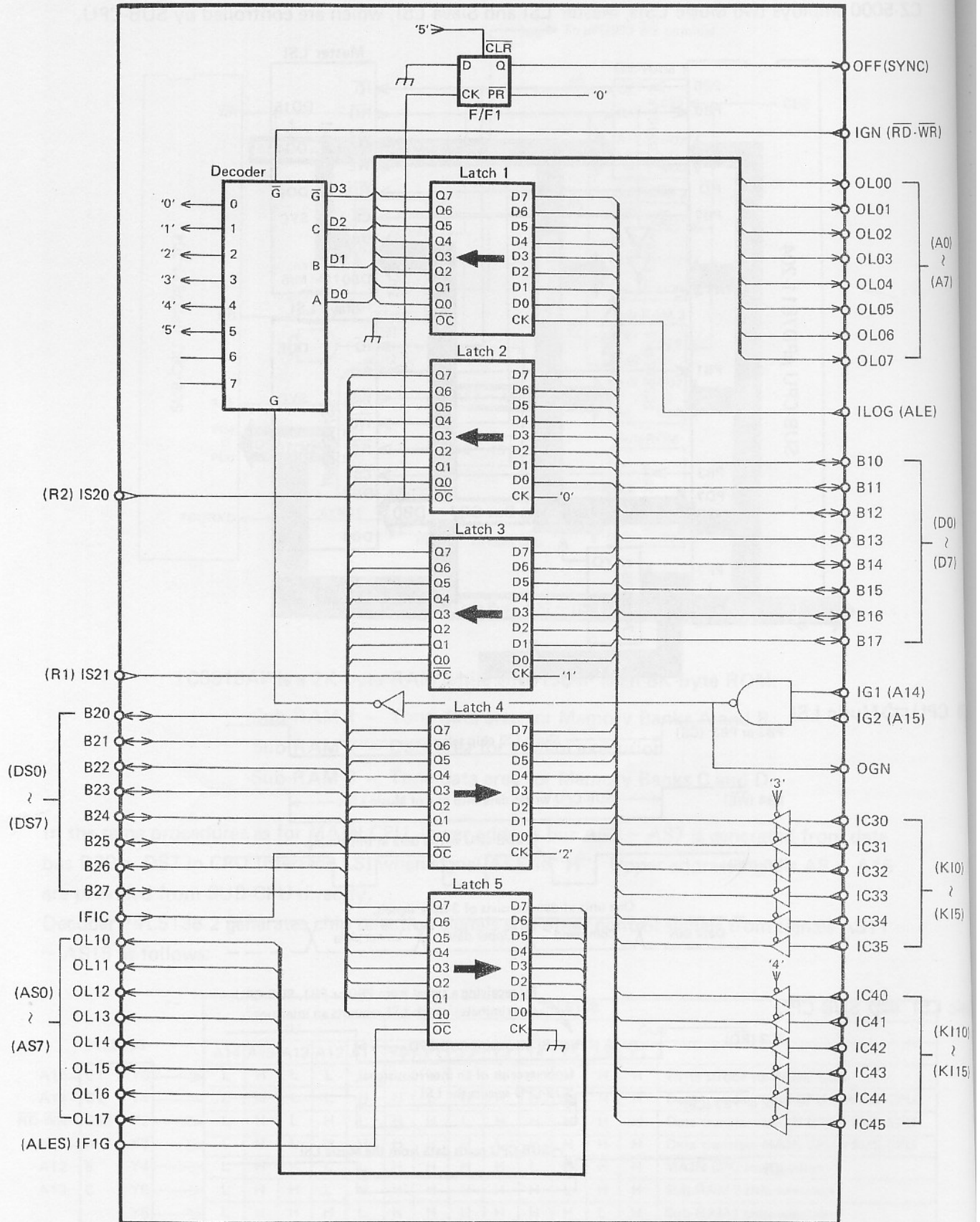
Internal block diagram of MB64H173
