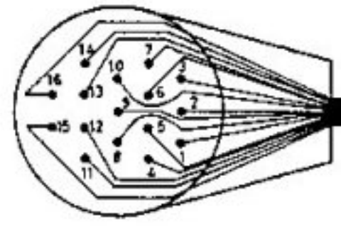
PEDAL-BOARD CONNECTOR (PLUG)
