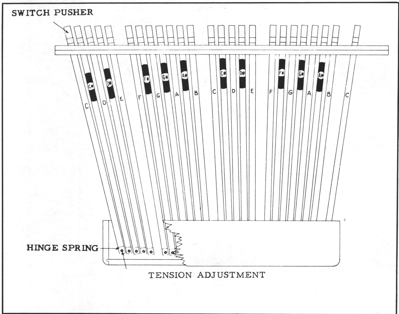
Figure 2-4. Pedal Keyboard
