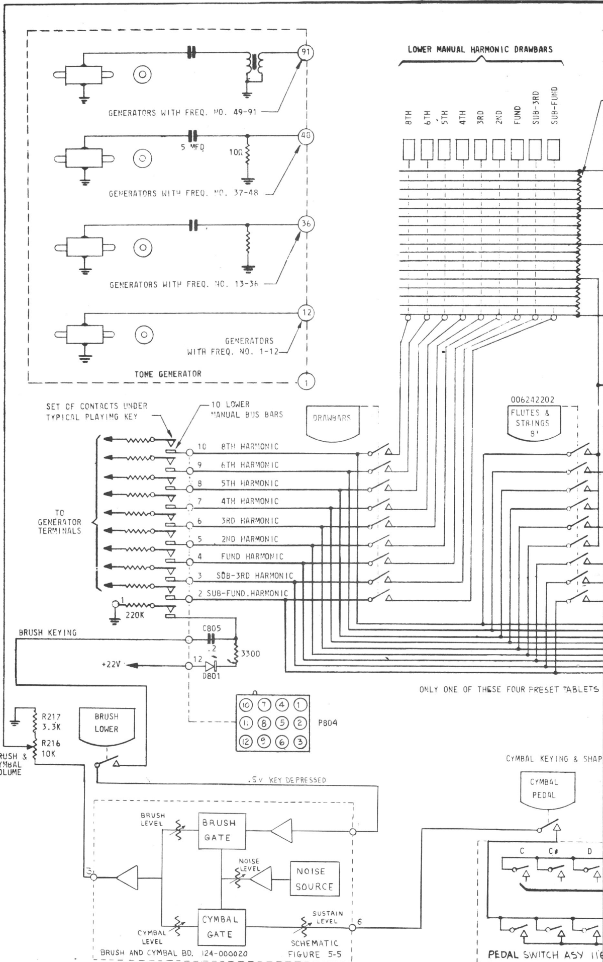
Figure 5-1. R-100 Organ, Schematic Diagram, Sheet 1 of 3
