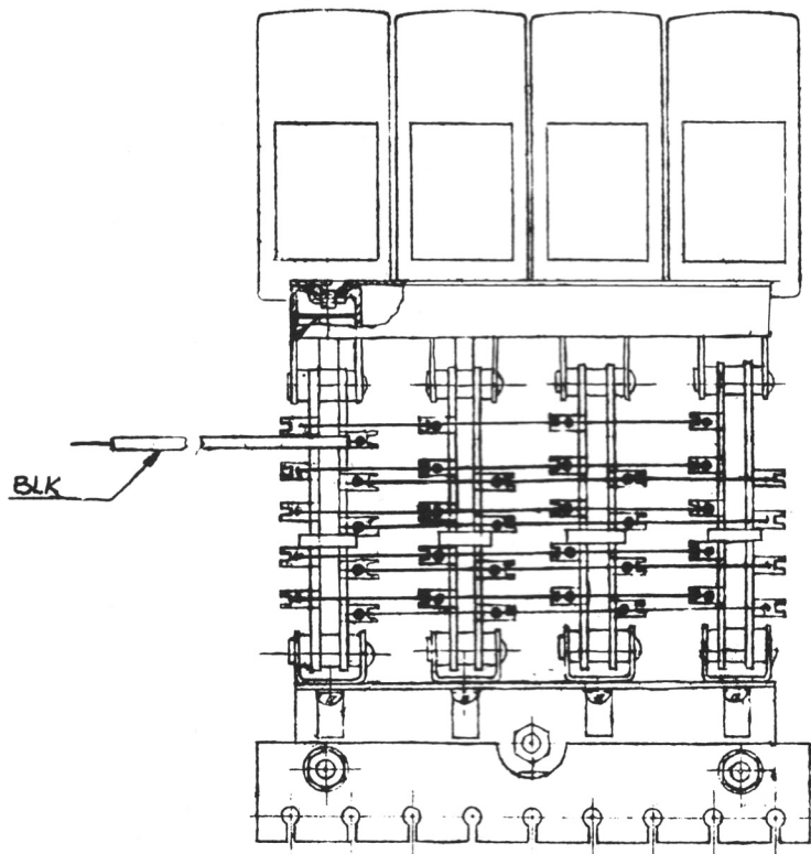
Figure 5-22. Upper Preset Switch Assembly, Wiring Diagram
