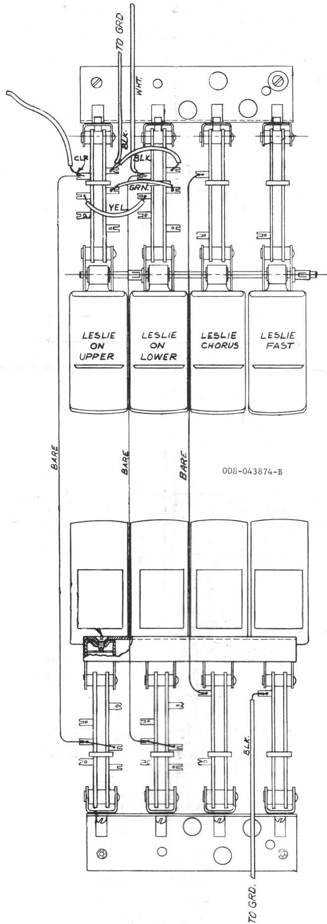
Figure 5-17. Leslie Switch Assembly, Wiring Diagram
