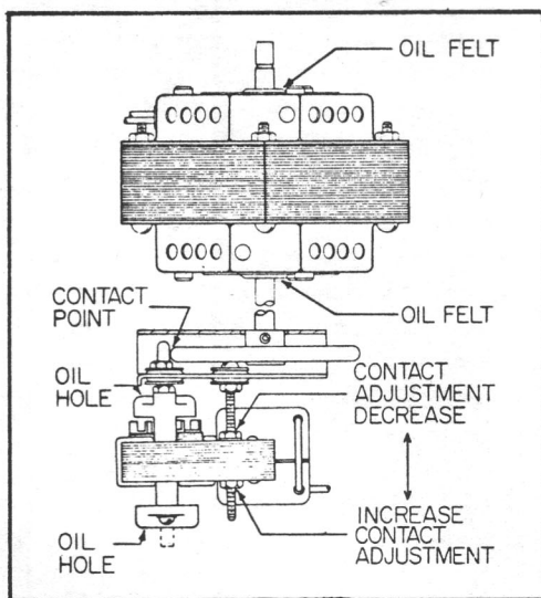
Figure 4-4. Leslie Motor Lubrication and Adjustments
