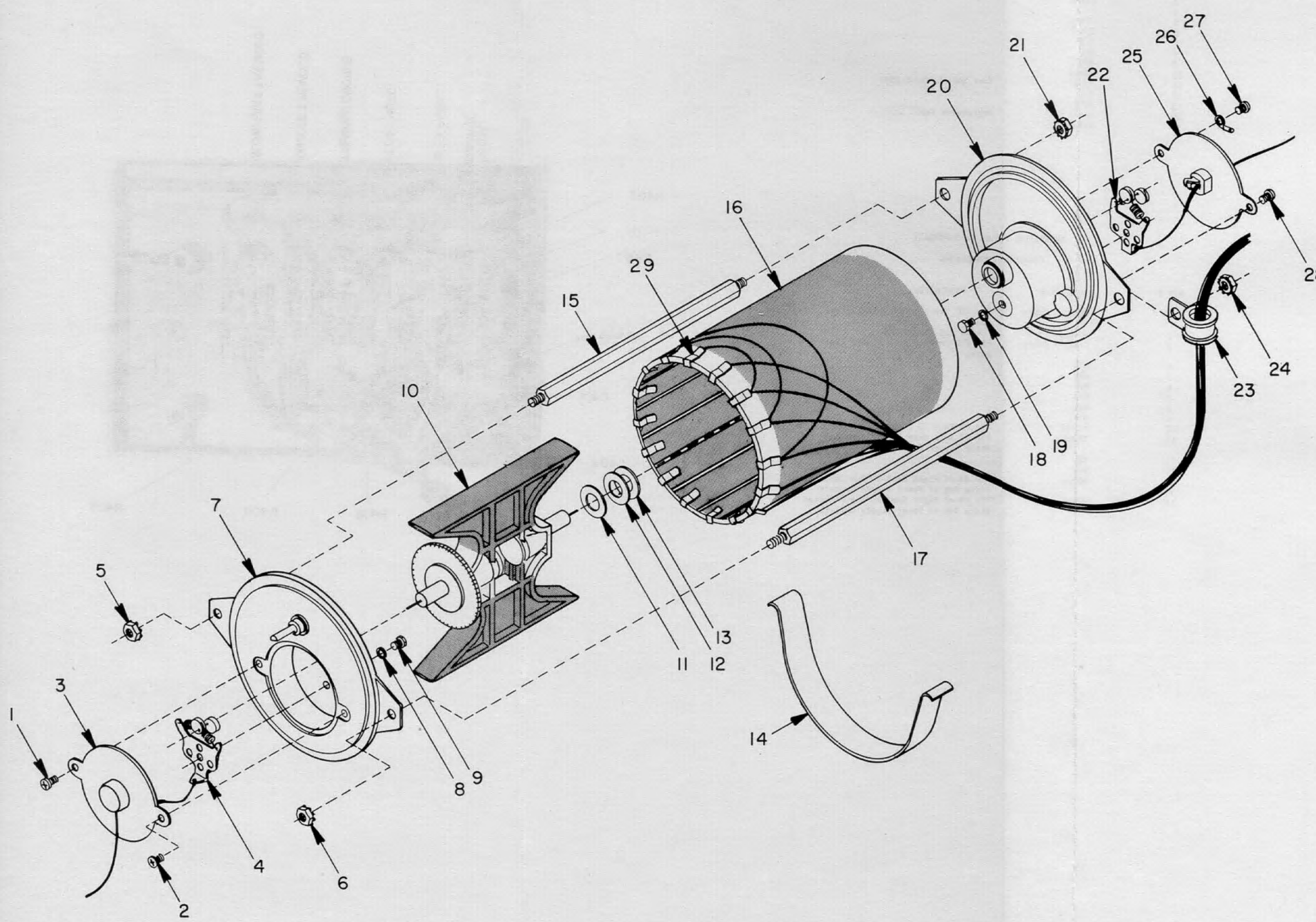
FIGURE 5-14 DRUM SCANNER 066-042874
