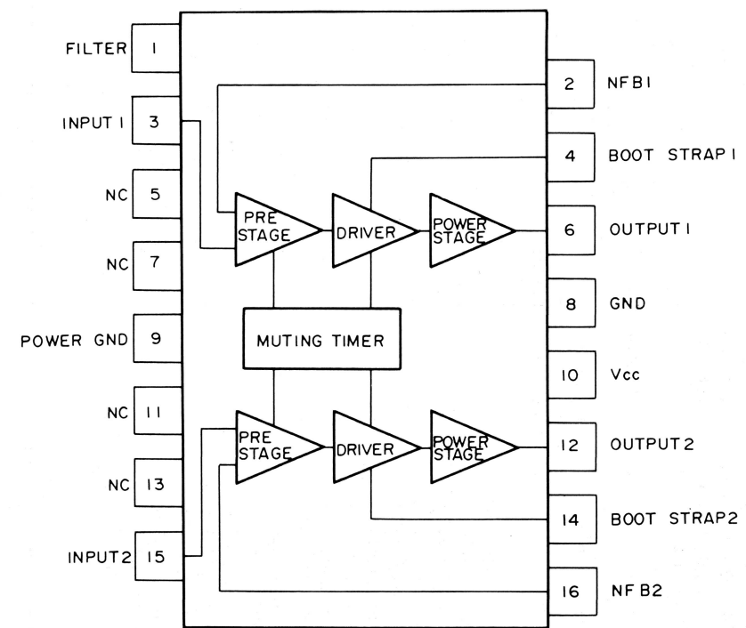
BLOCK DIAGRAM
