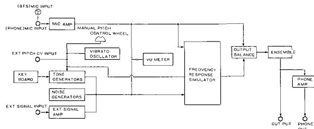
▲KORG VOCODER VC-10 BLOCK DIAGRAM
