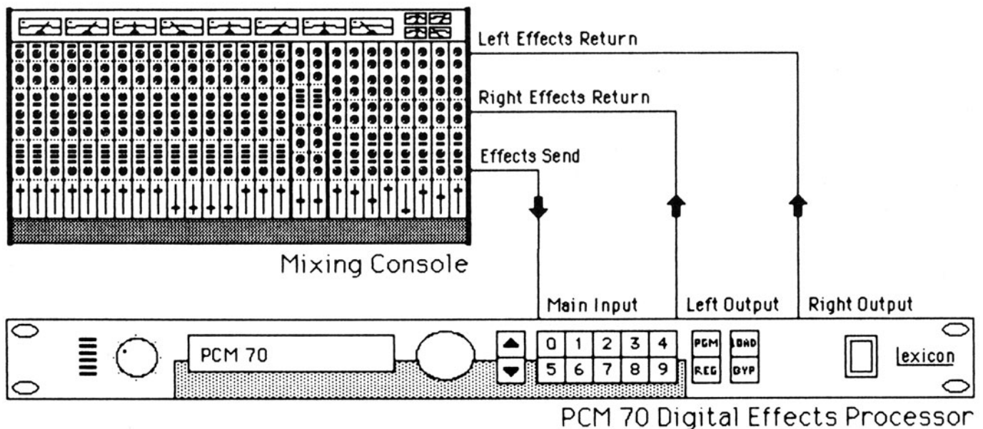
Figure 1.1. Connection to mixing console.
