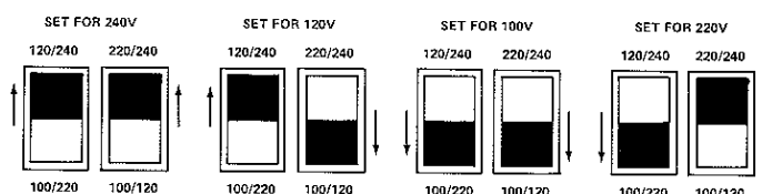
Figure 3-1 – Setting the Voltage Changeover Switches
