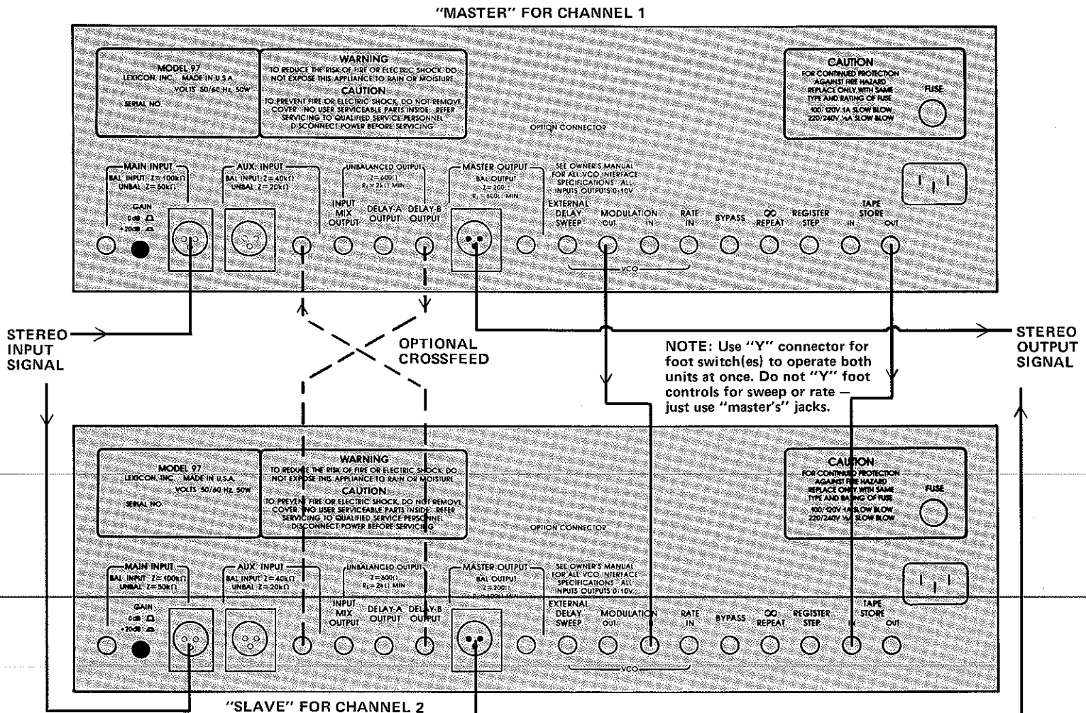
Figure 6-6 — Processing a Stereo Program with Cross-Coupling between Two Model 97s
