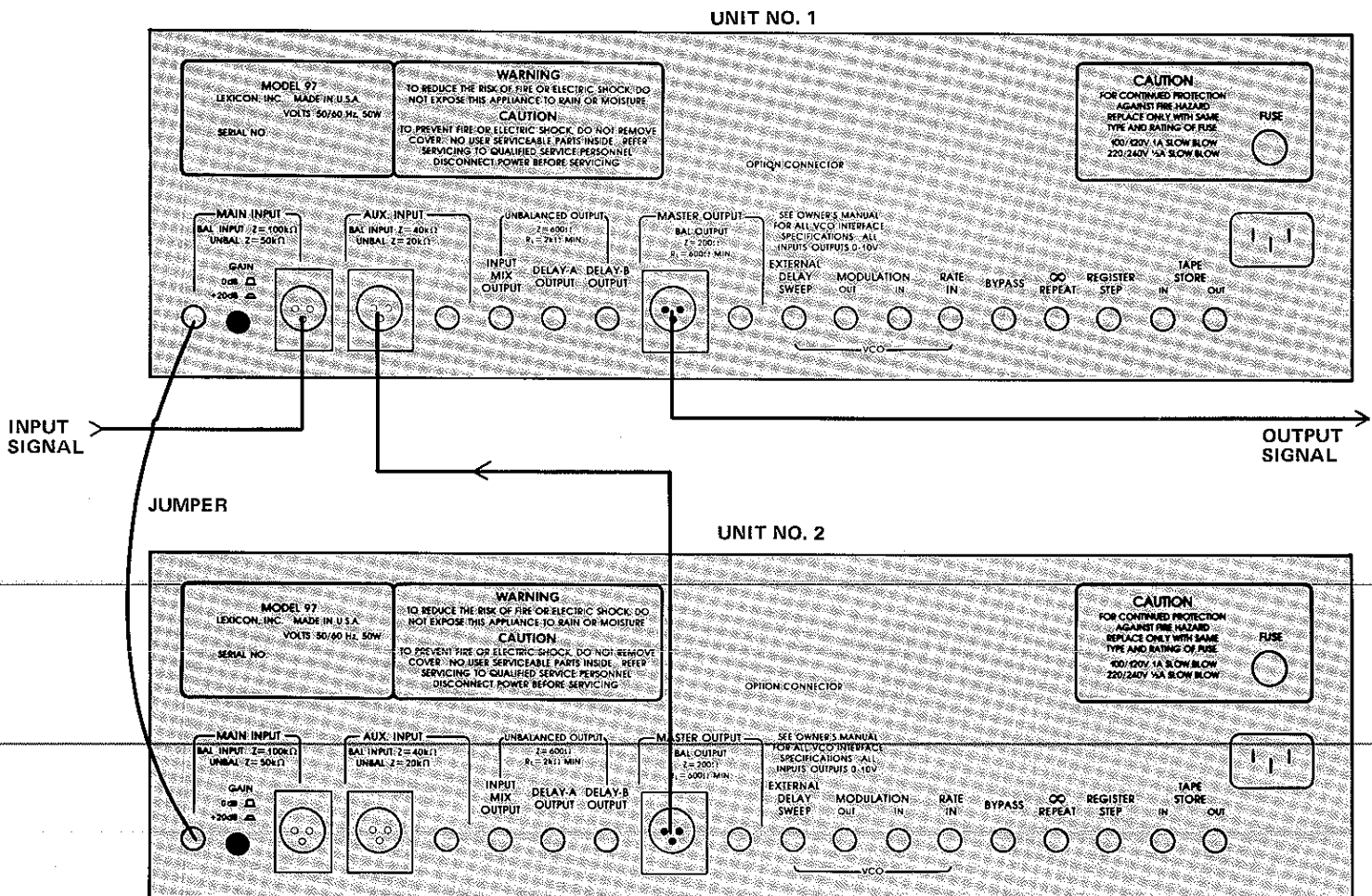
Figure 6-8 — Connection of Two Model 97s for Deep Tape Phasing (Flanging) Effects (See accompanying text.)
