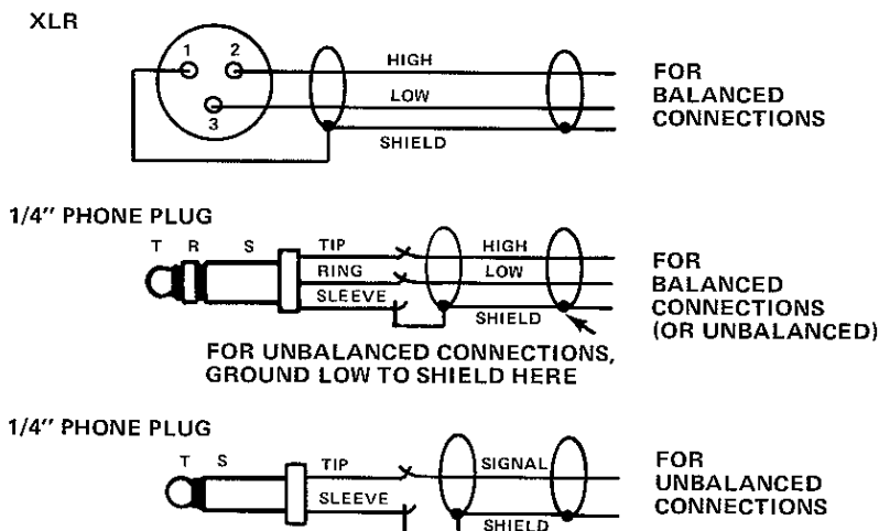
Figure 3-2 – Typical Wiring of Audio Input and Output Connections
