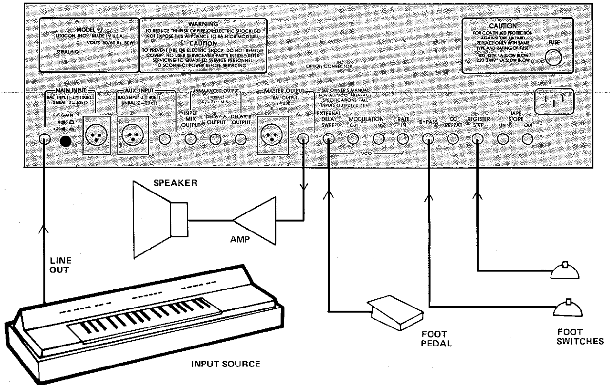
Figure 6-2 – Basic Mono Setup for Electronic Keyboard Player
