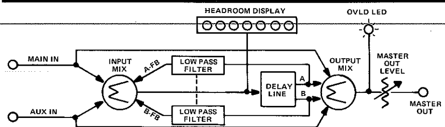
Figure 4-1 — Input and Output Mix Section Block Diagram
