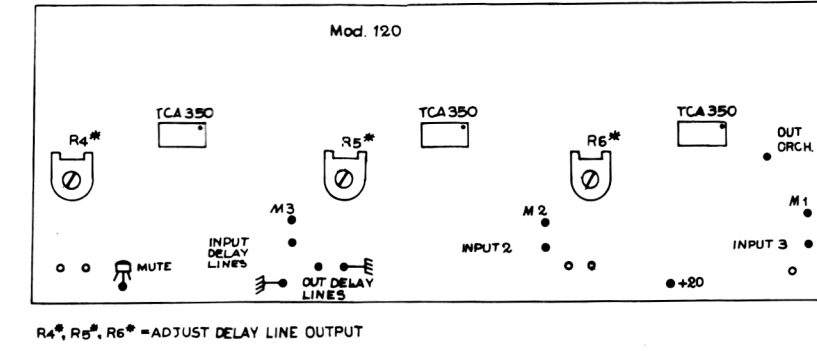
R4*, R5*, R6* = ADJUST DELAY LINE OUTPUT
