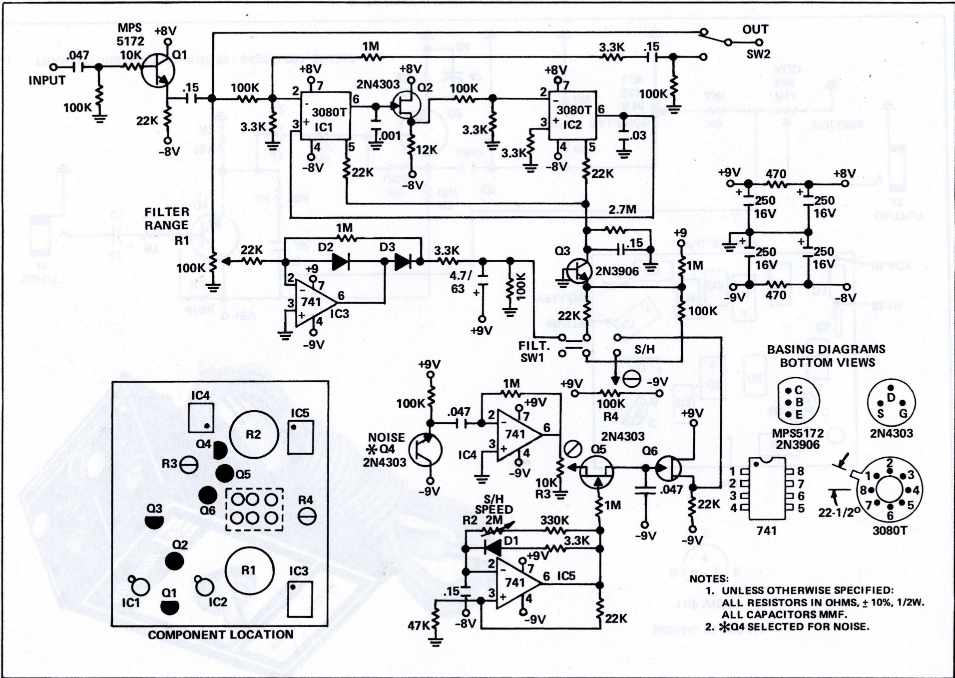
FILTER - SAMPLE AND HOLD MODEL FSH-1A
