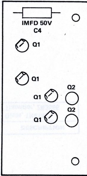
BOARD TOP VIEW
