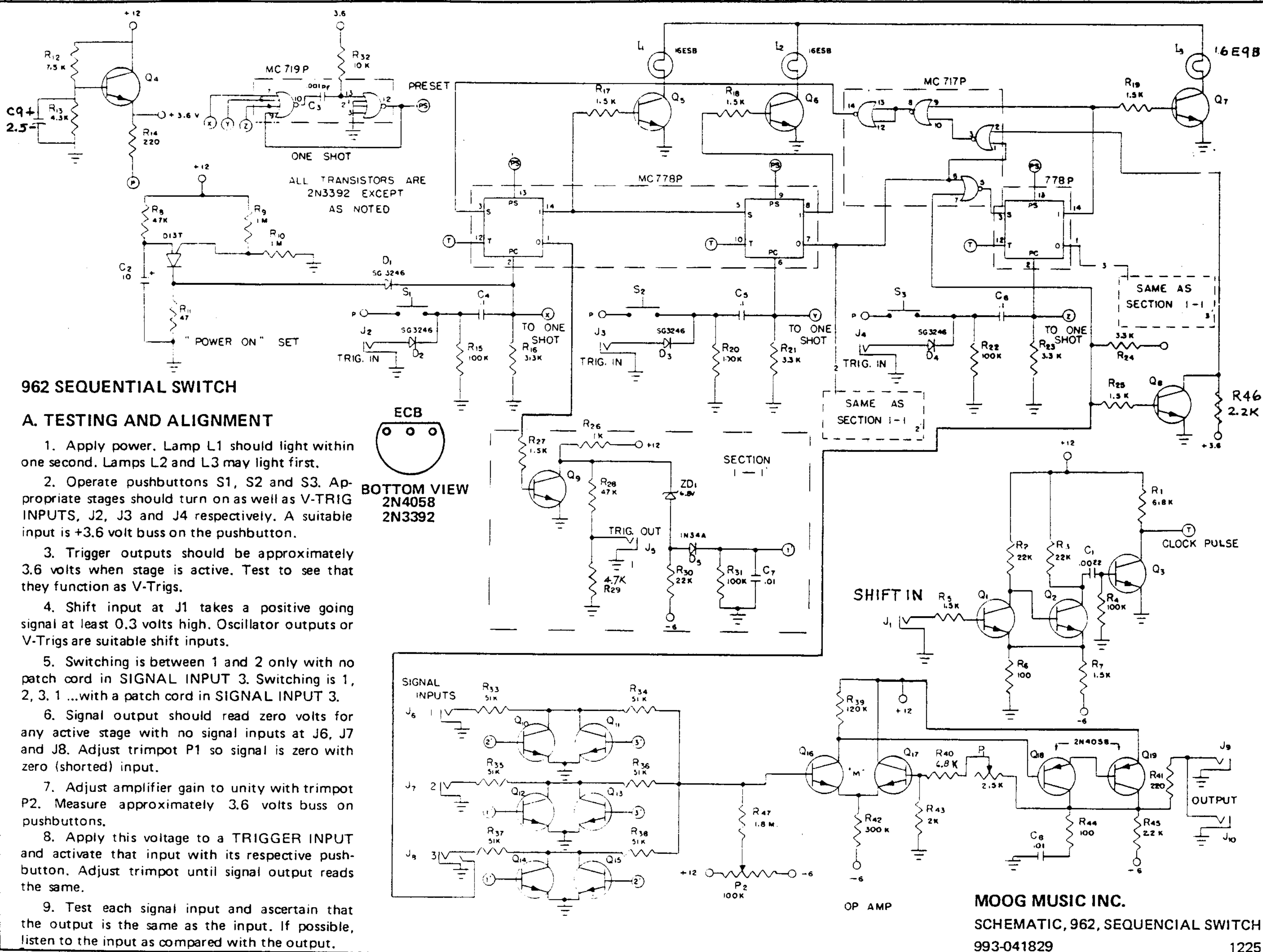
FIGURE 35. SEQUENTIAL SWITCH MODEL 962
