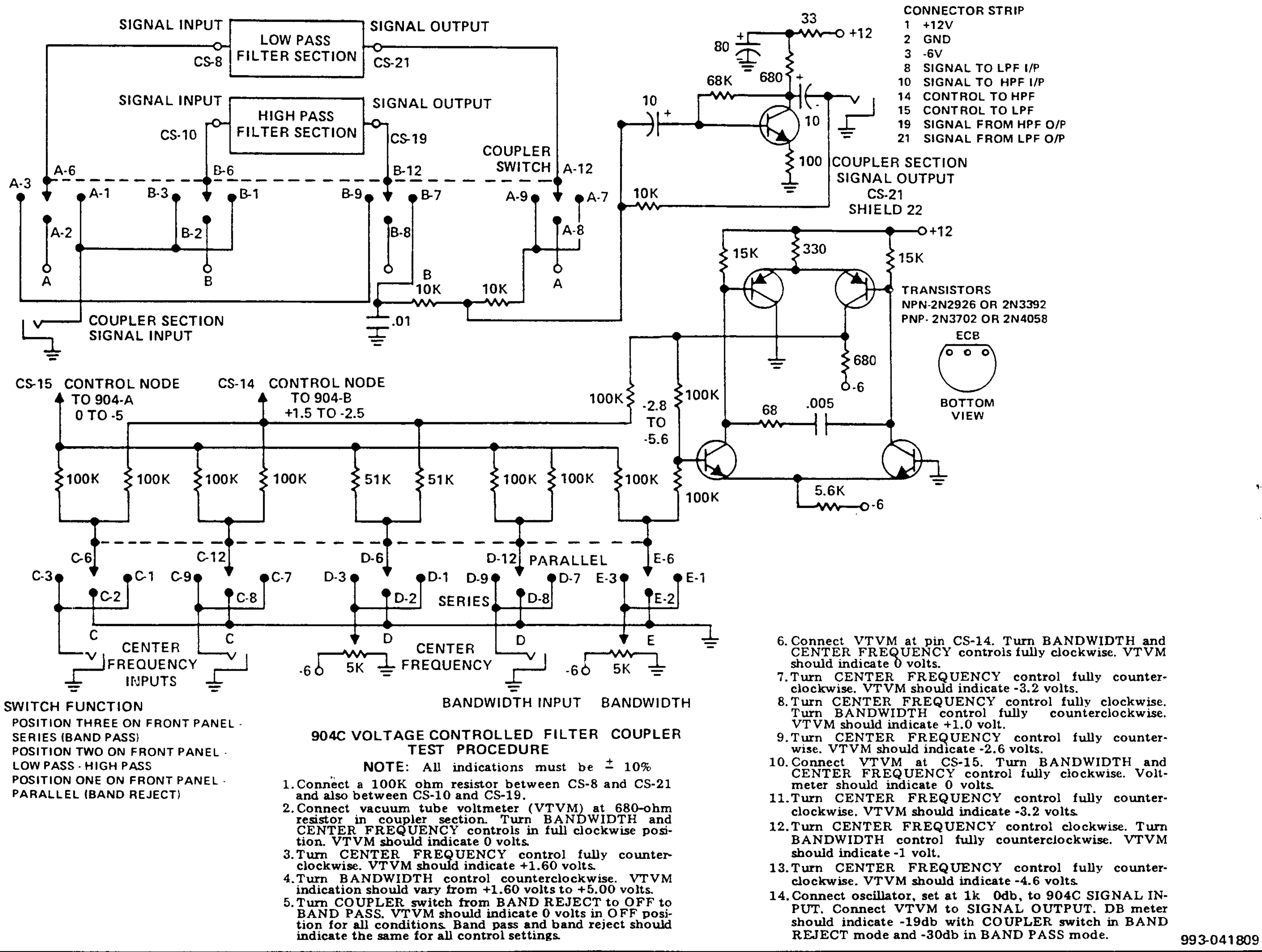
FIGURE 13 VOLTAGE CONTROLLED FILTER COUPLER MODEL 904C
