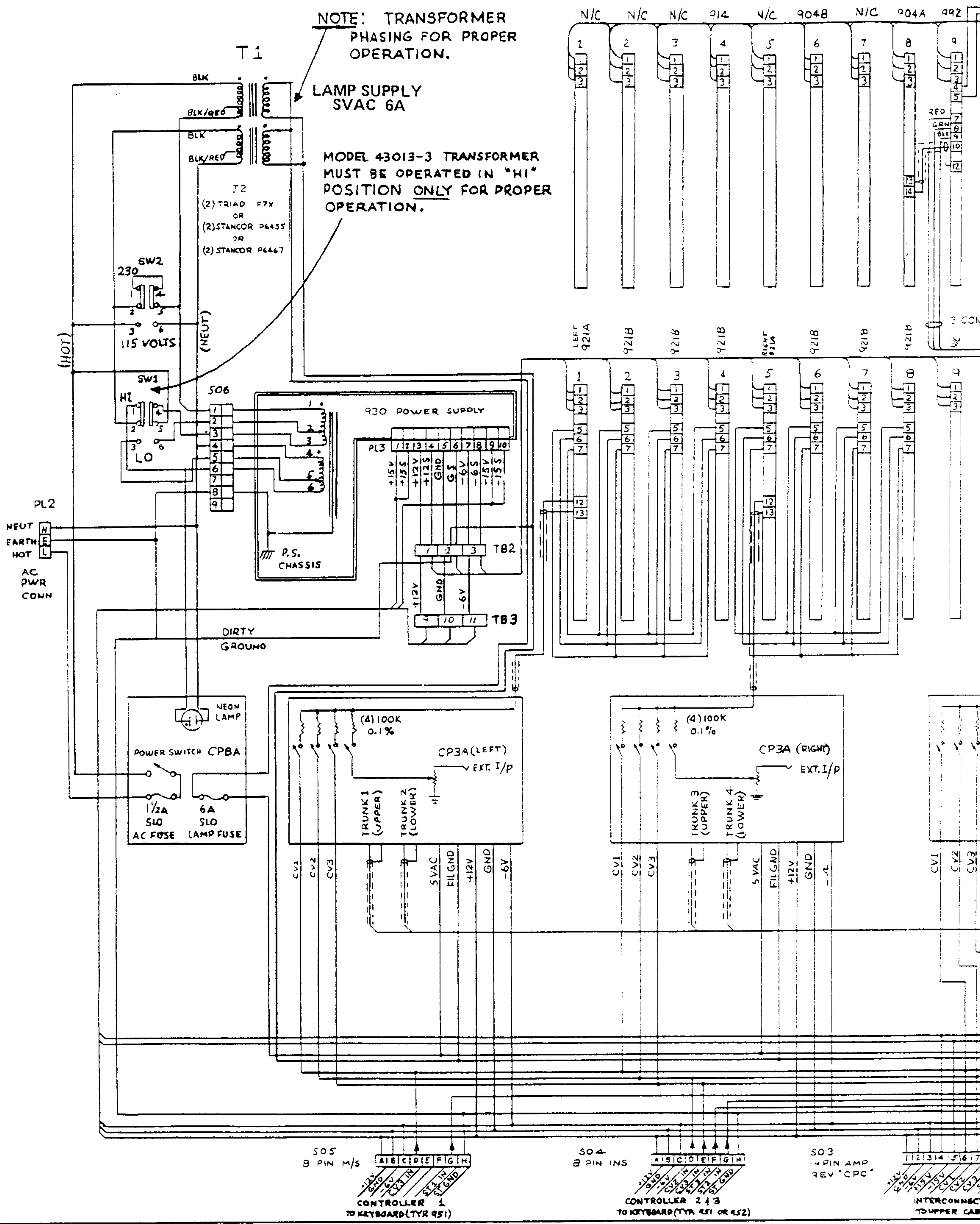
FIGURE 48 CABINET WIRING, SYSTEM 55
