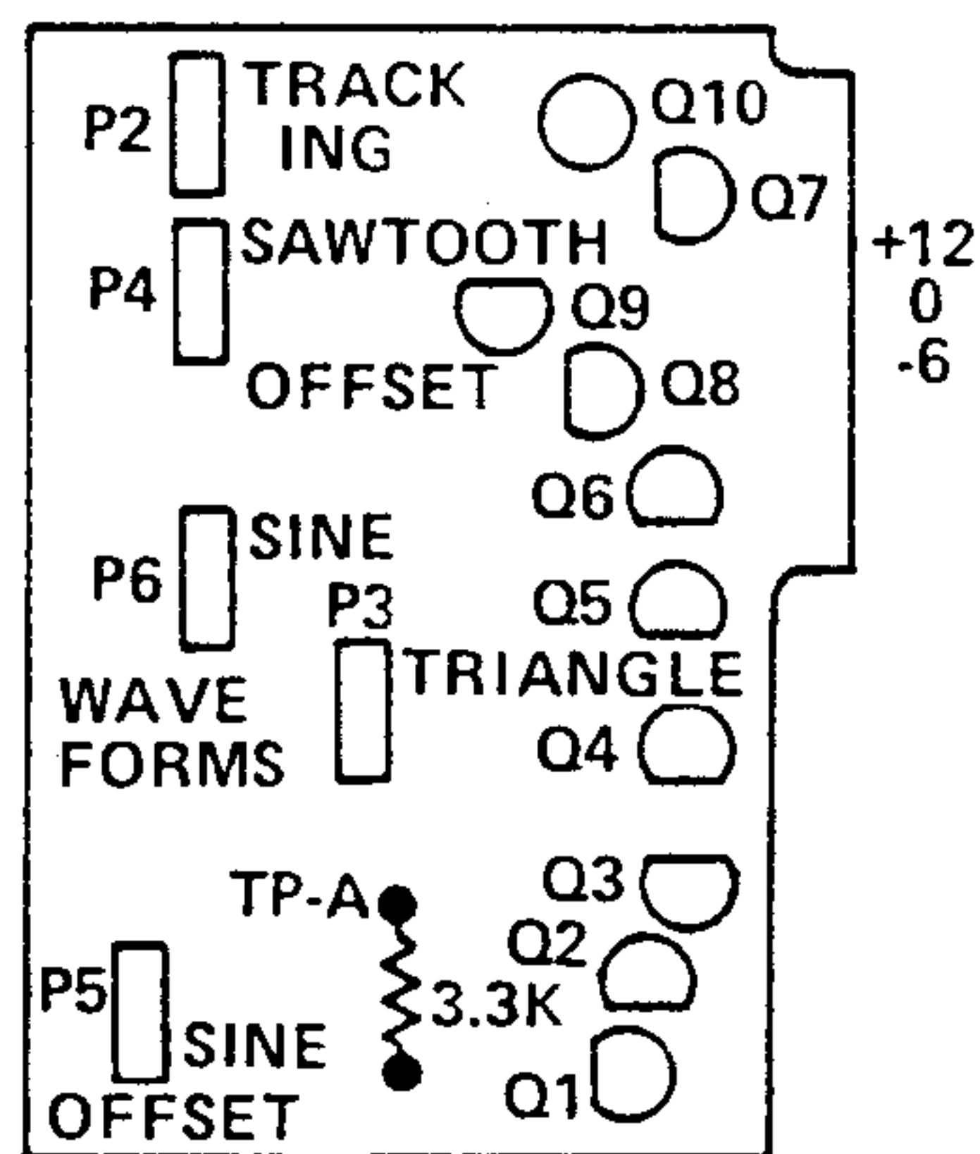
ADJUSTMENT LOCATION DIAGRAM
