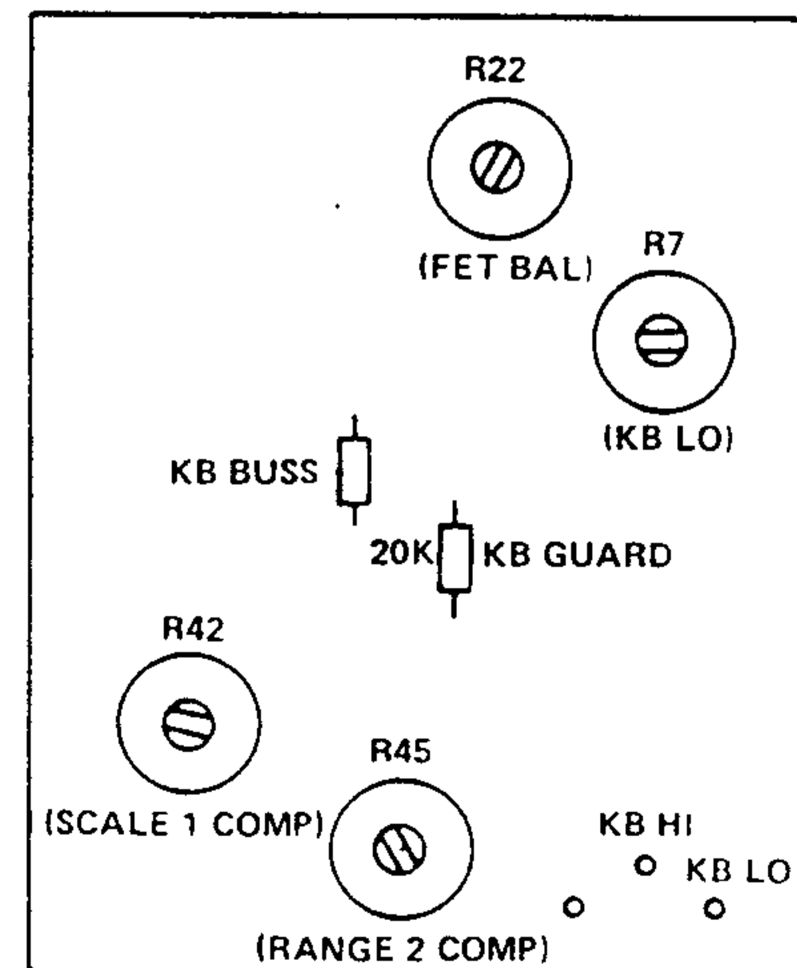
952 ADJUSTMENT LOCATIONS
