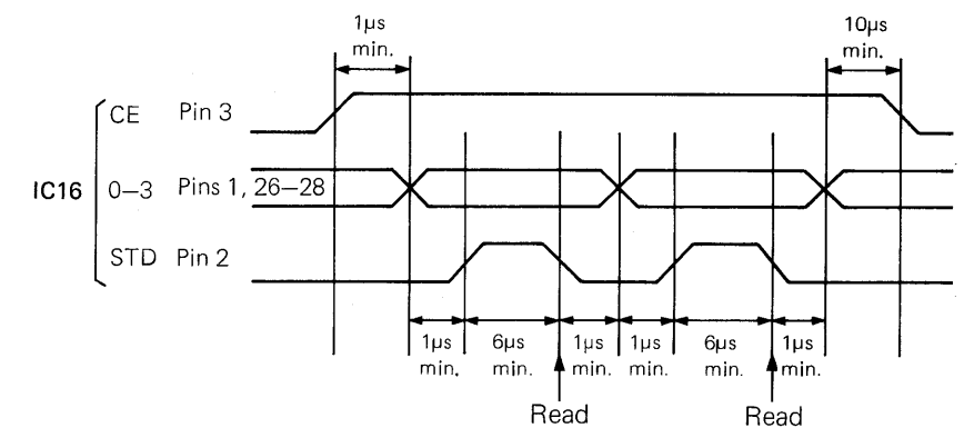
Data Latch Timing Chart (IC13 to IC16)
