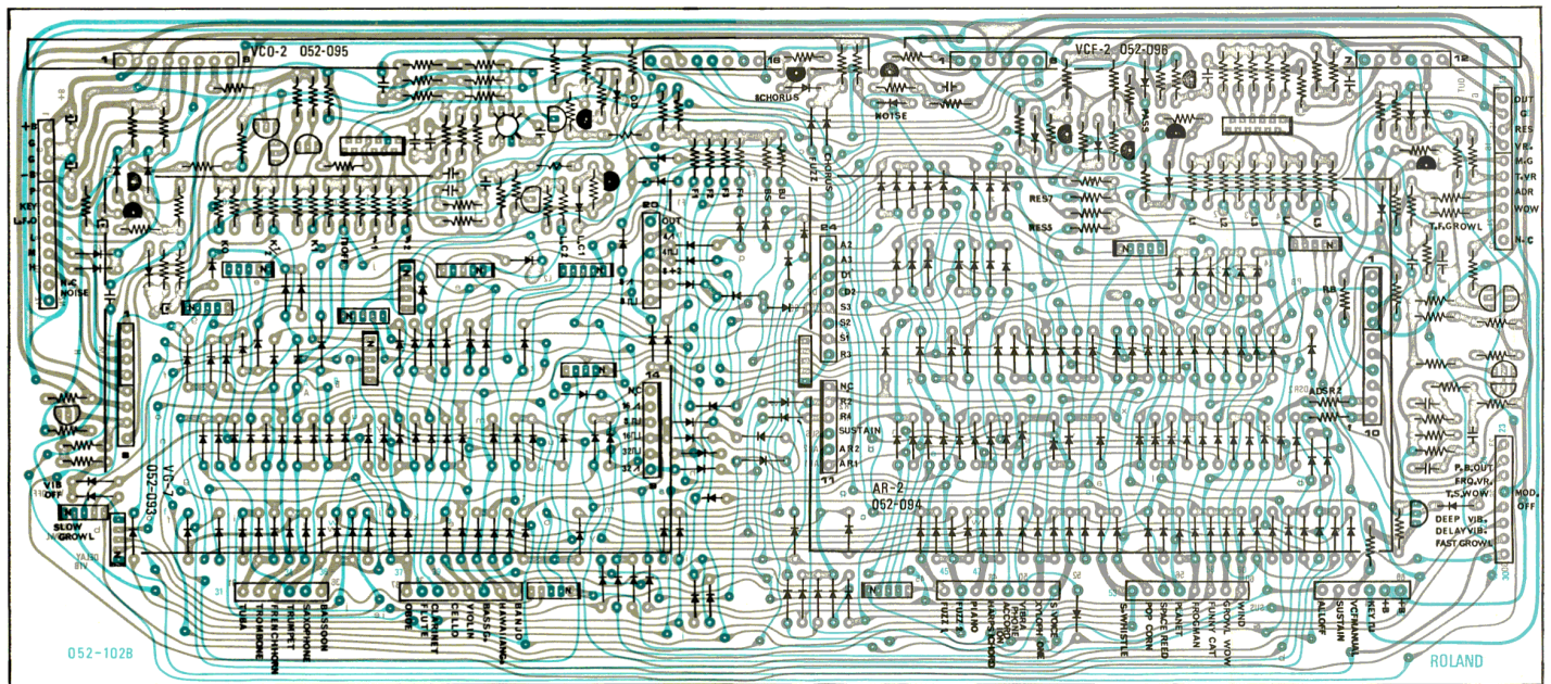
9-5. Both Side Circuit Patterns of MX-1 Board
