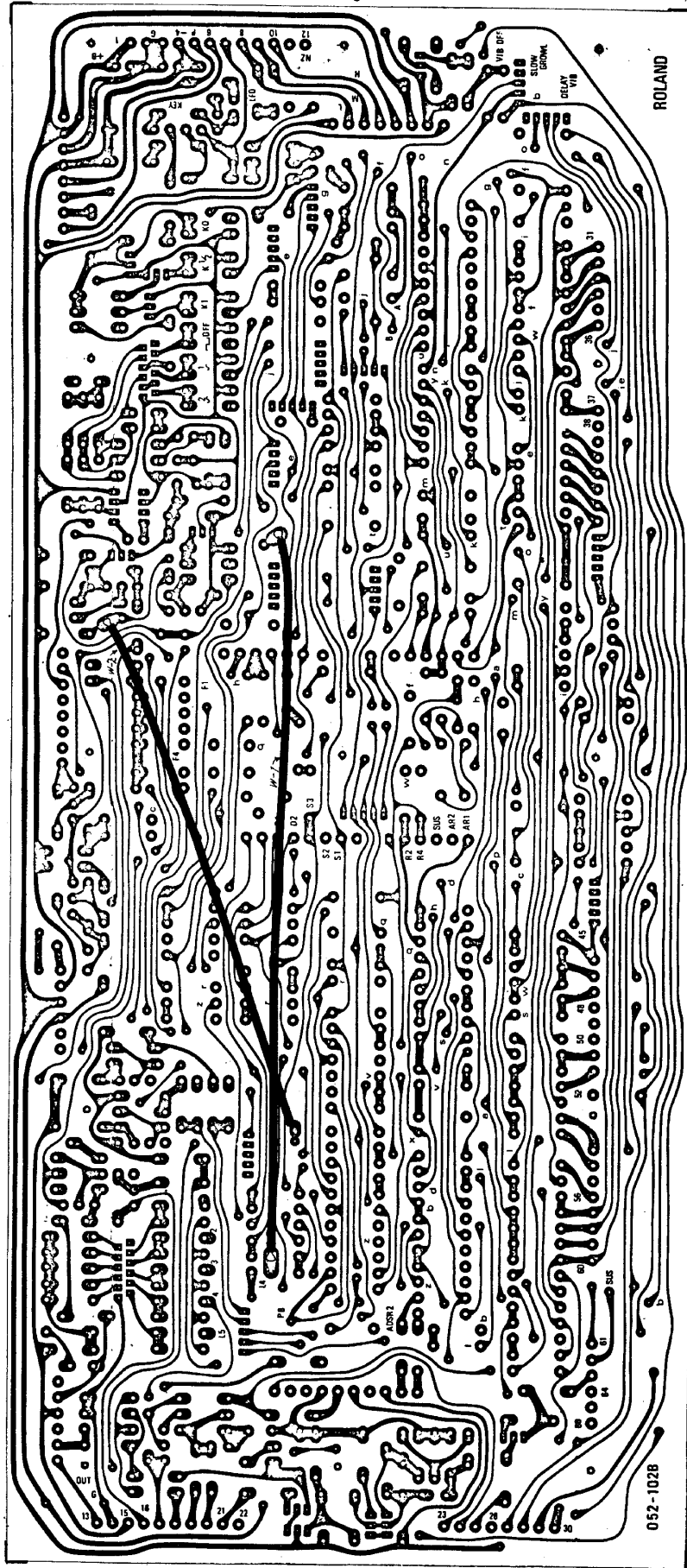
9-4. Rear Side of MX-1 Board
