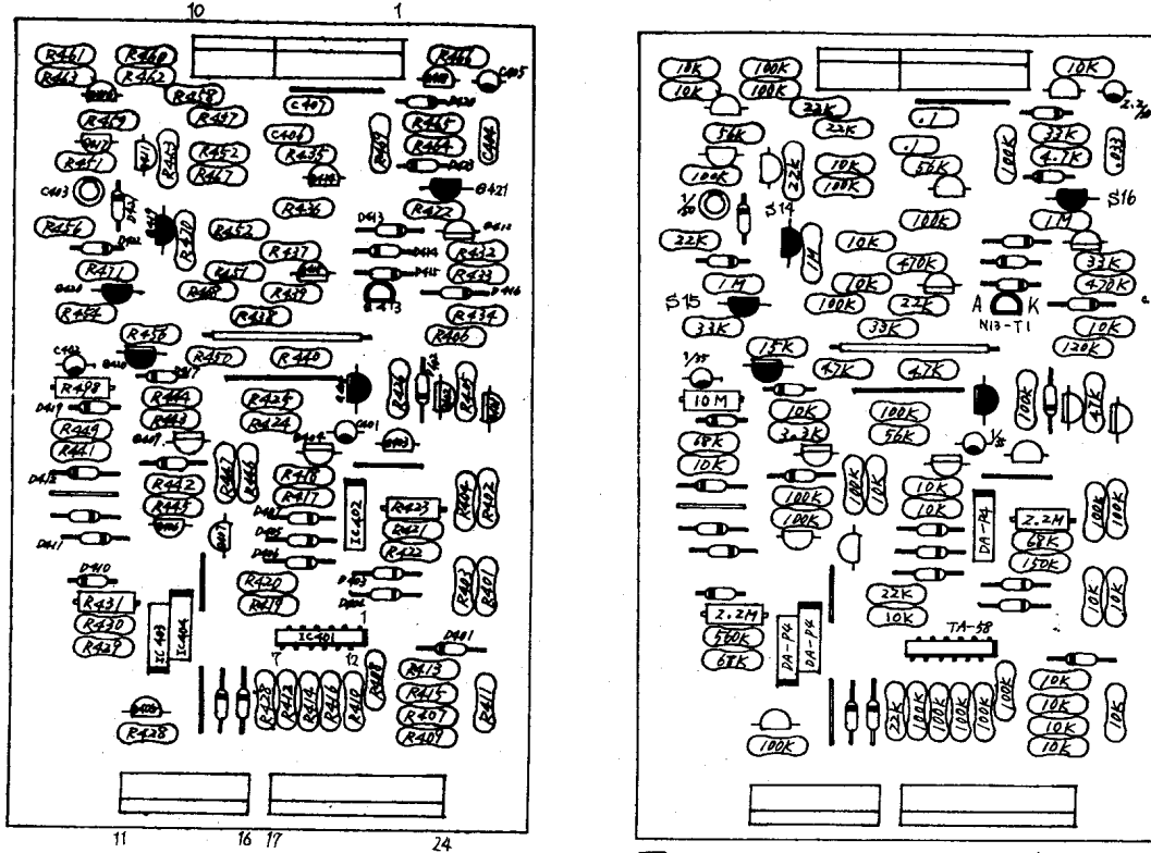
7-2. AR-2 Circuit Diagram
