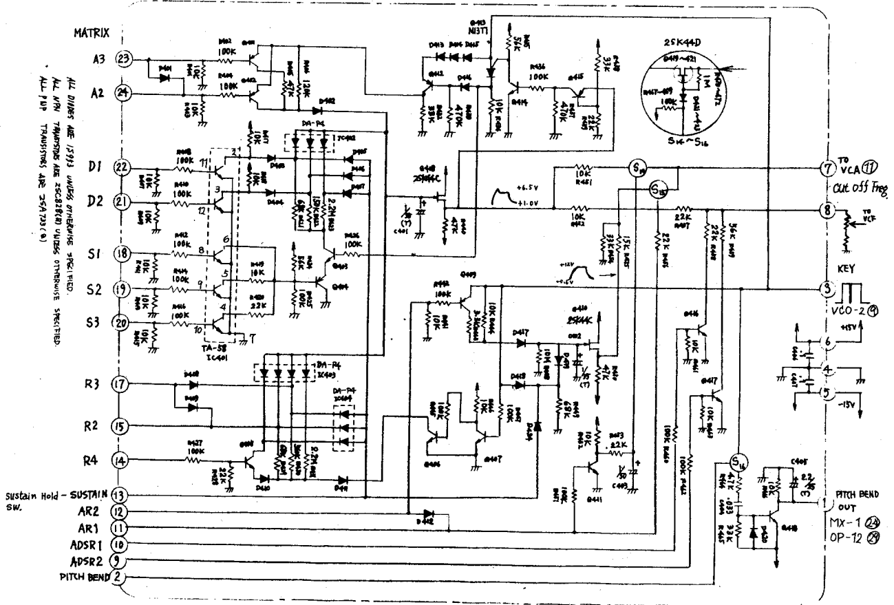
7-2. AR-2 Circuit Diagram
