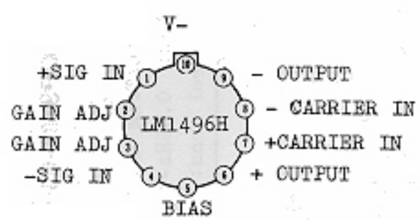
LM1496 balanced modulator-demodulator
