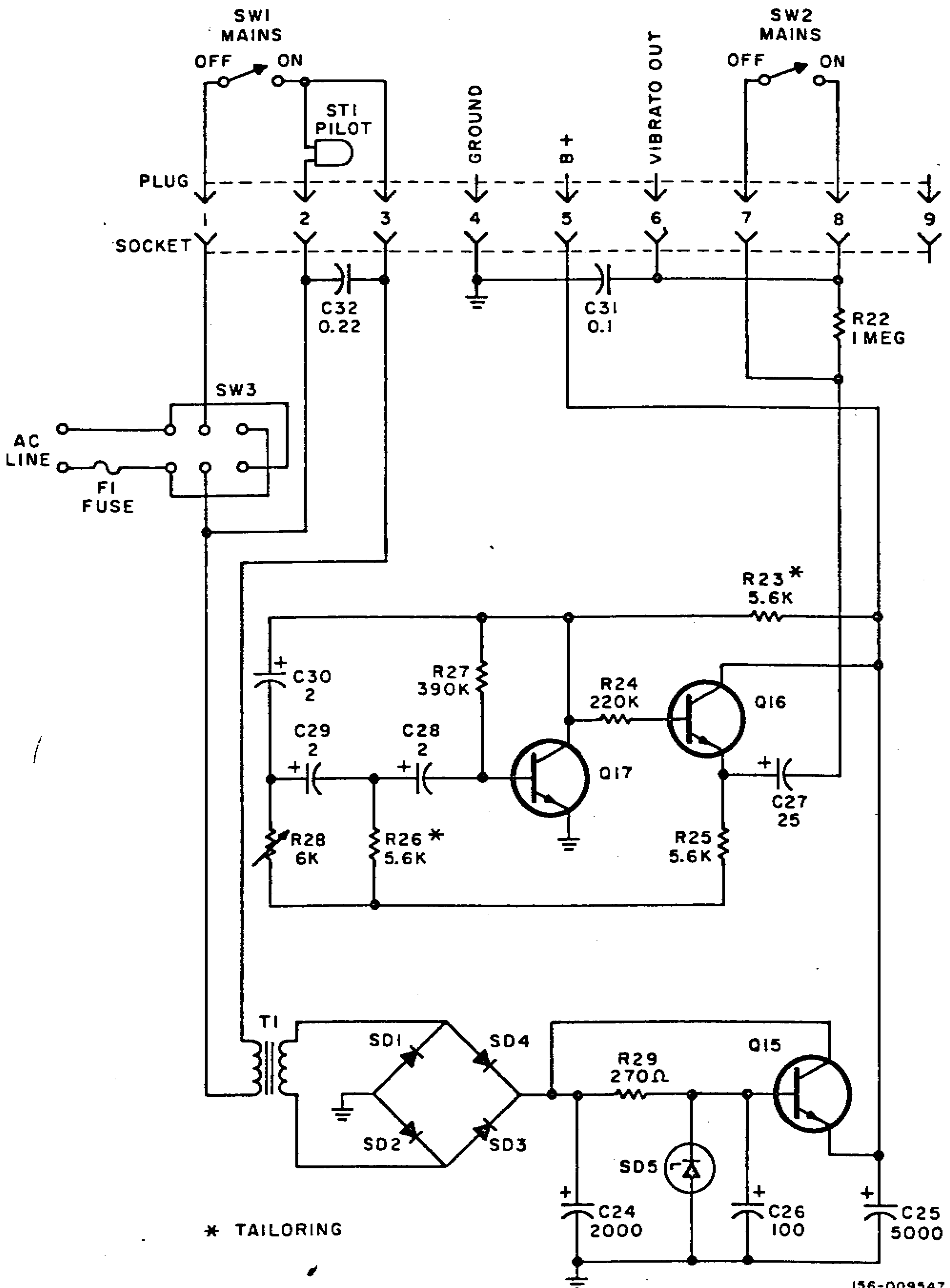
Figure 23. Power Supply Schematic
