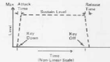
LEVEL VS TIME
