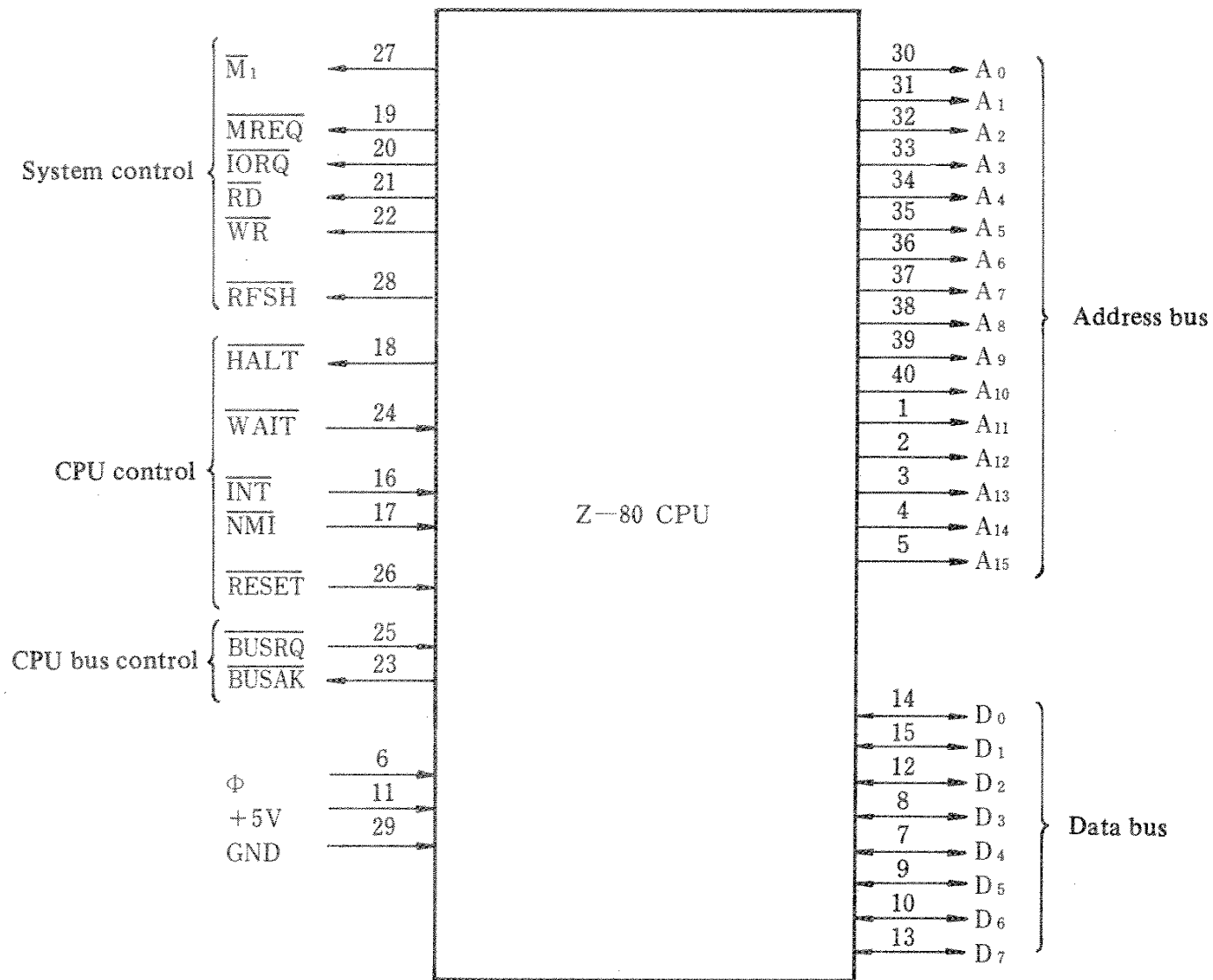
Fig. 20 Z-80A CPU Pin Layout
