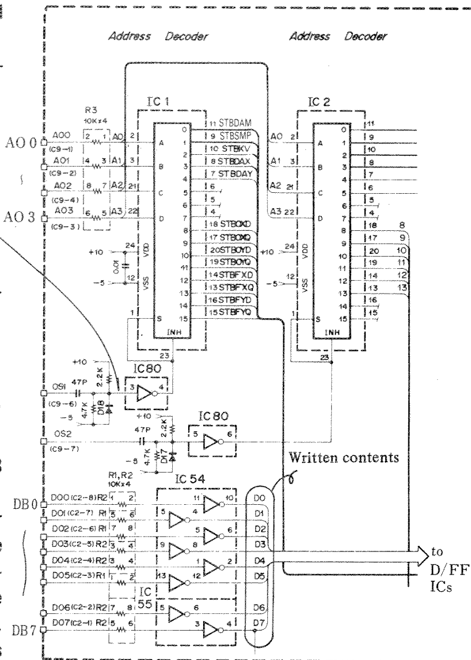
Fig. 7 Address Decoder Circuit
