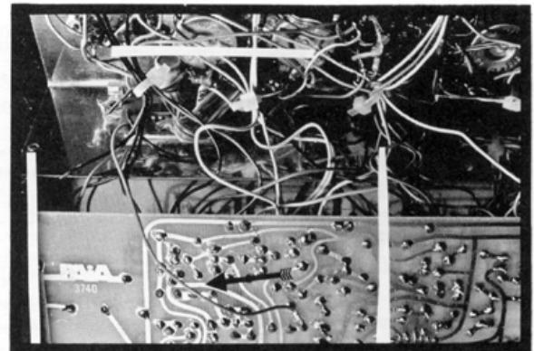
Figure 5: VCO connection.
