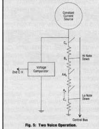
Fig. 5: Two Voice Operation.
