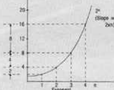
Fig. 3: Exponential Scale.
