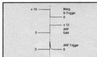
Fig. 1: Synthesizer Timing Pulses.
