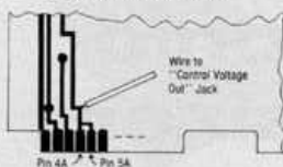
Fig. 4: Minimoog Board No. 2.
