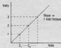
Fig. 2: Linear Control Voltage.
