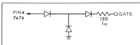
Optional gate protection circuit for negative voltages
