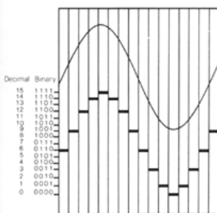
Figure One: Analog sinewave and digital equivalent.
